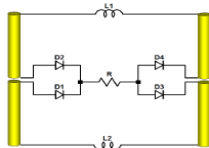
Fig 4(a): Proposed full-wave rectification system
