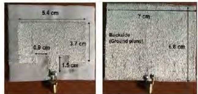
Fig 8: Textile-based antenna
